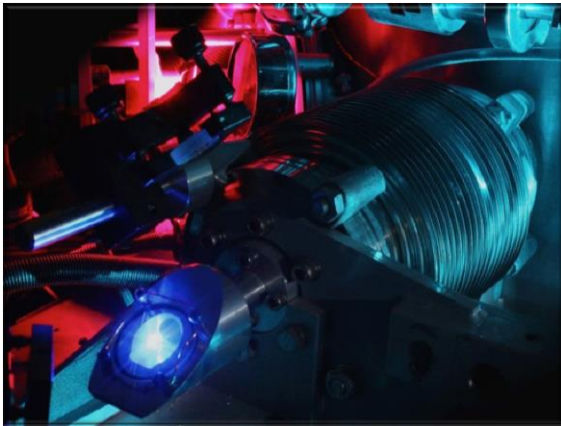
Figure: This photo shows the vacuum chamber used to measure the 2S-4P transition frequency in atomic hydrogen. The purple glow in the back stems from the microwave discharge that dissociates hydrogen molecules into hydrogen atoms. The blue light in the front is fluorescence from the ultraviolet laser that excites the atoms to the 2S state. The turquoise blue glow is stray light from the laser system used to measure the frequency of the 2S-4P transition. (Photo: MPQ)
